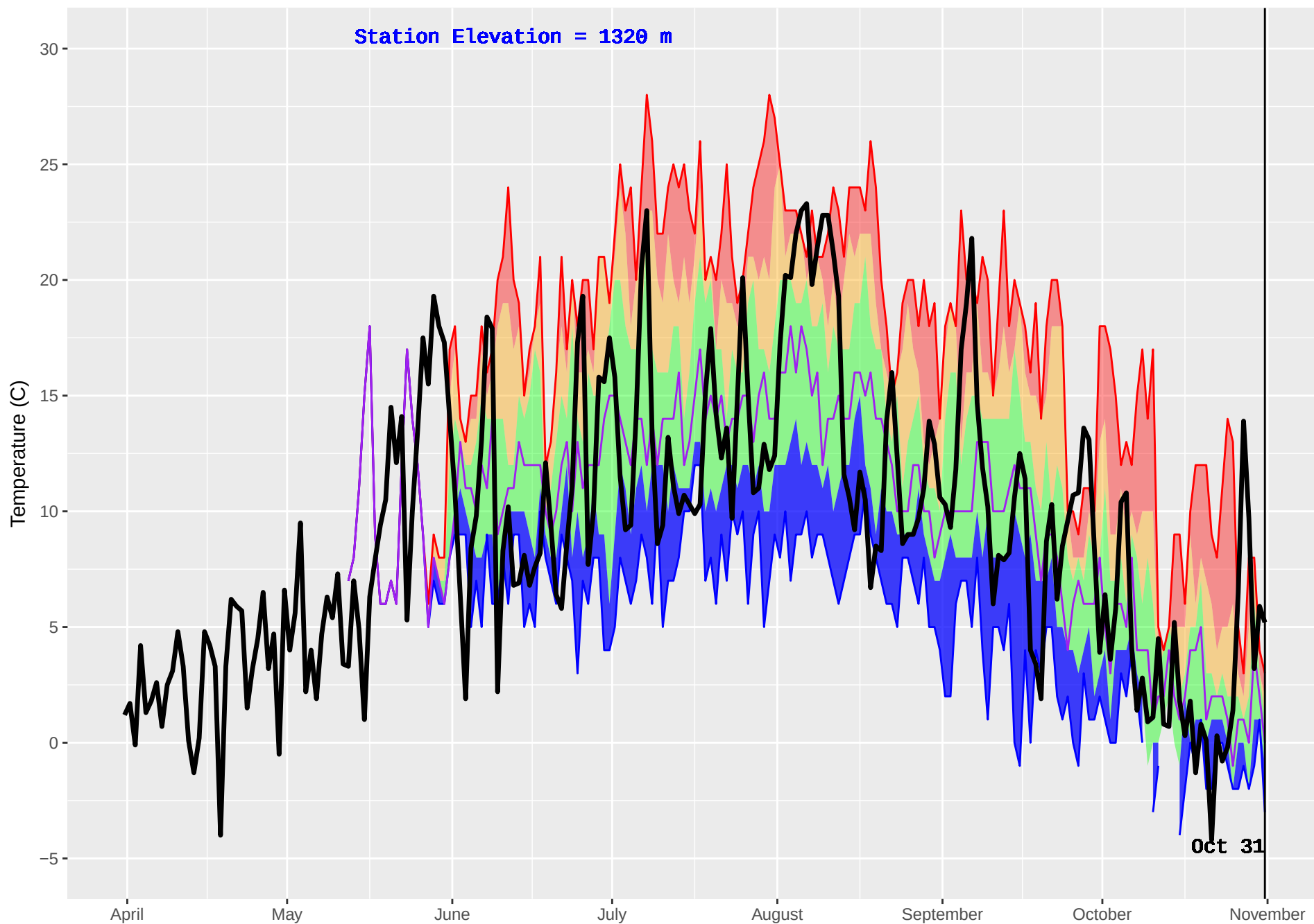
PINE CREEK (938) : Historical (2006–2016) and Current (2017) Noon Temperature
