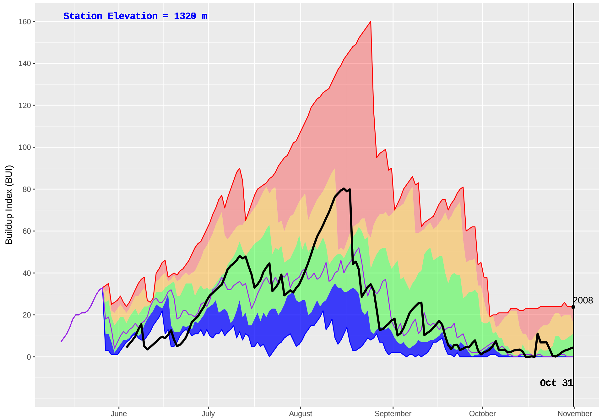
PINE CREEK (938) : Historical (2006–2016) and Current (2017) Noon Buildup Index (BUI)
